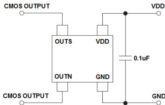
Figure 1, Typical Application Circuit of AS1826A
